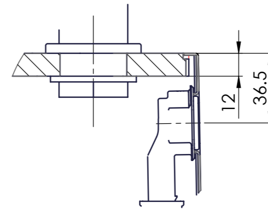
X (1:2)
